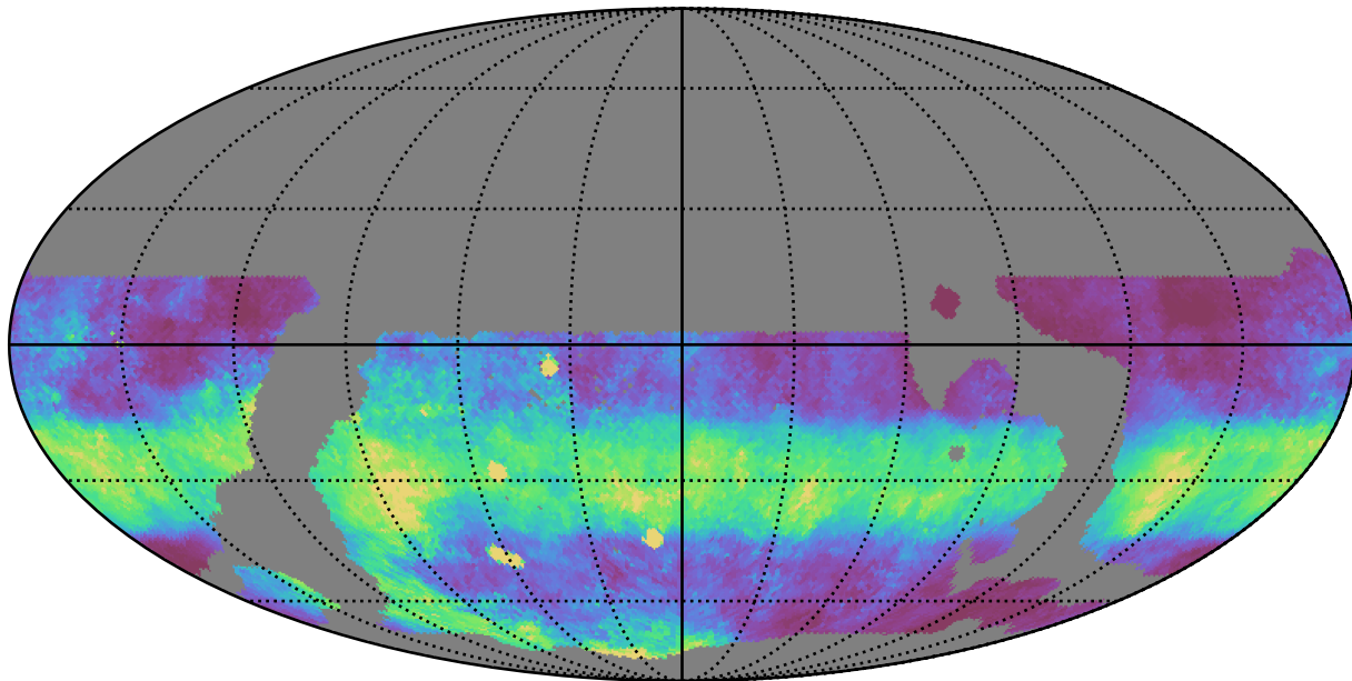
weather_cloudso35v3.4_10yrs WFD z band: Median normairmass
