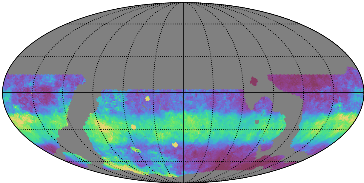
weather_cloudso35v3.4_10yrs WFD y band: Median normairmass
