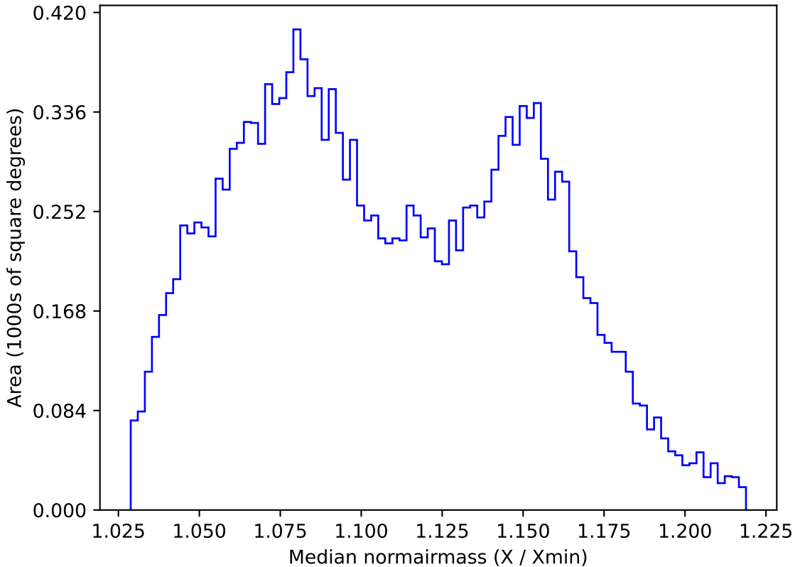
weather_cloudso35v3.4_10yrs WFD y band: Median normairmass
