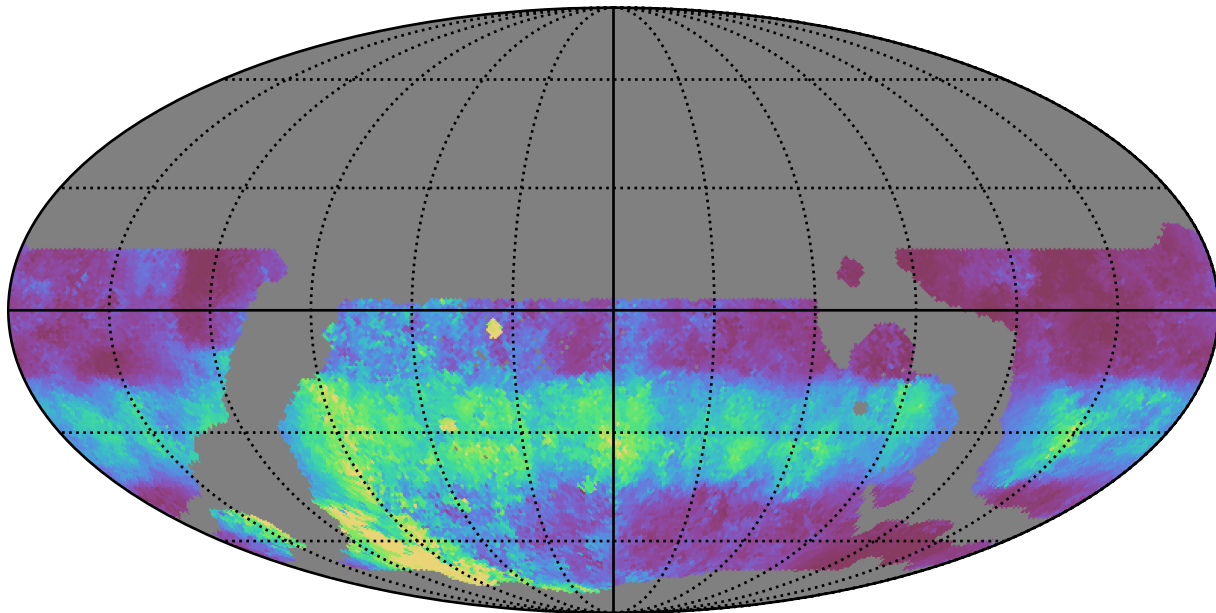
weather_cloudso35v3.4_10yrs WFD u band: Median normairmass
