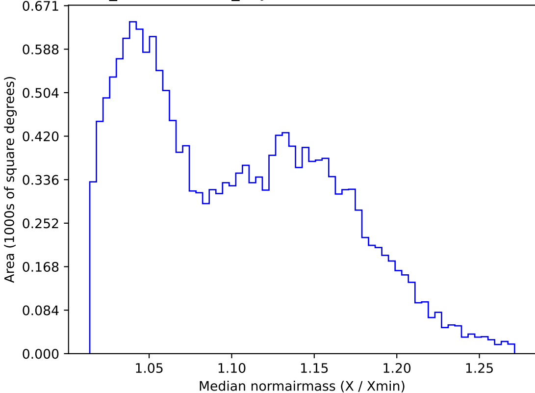
weather_cloudso35v3.4_10yrs WFD u band: Median normairmass
