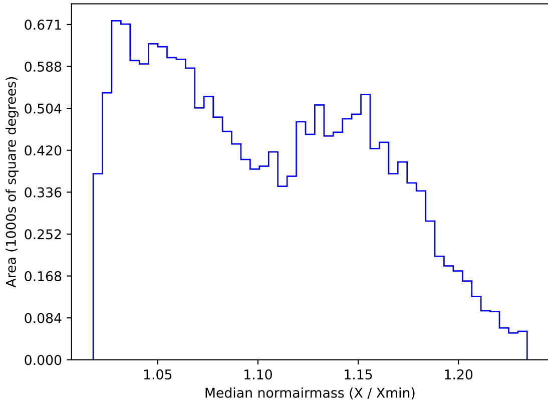
weather_cloudso35v3.4_10yrs WFD g band: Median normairmass
