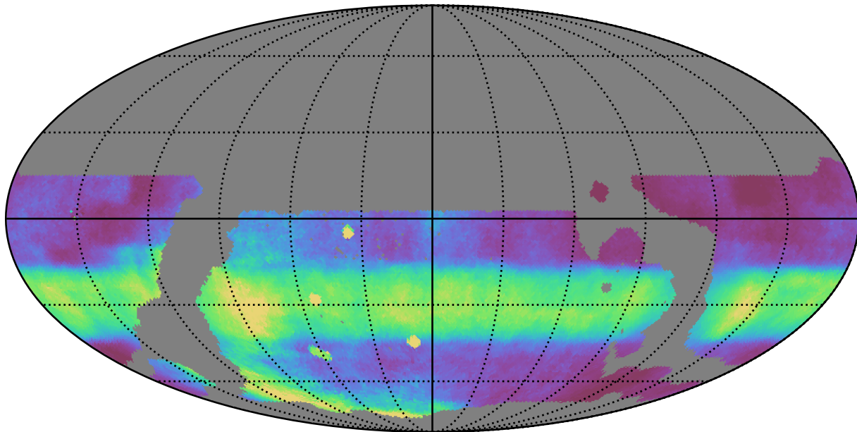
weather_cloudso35v3.4_10yrs WFD all bands: Median normairmass
