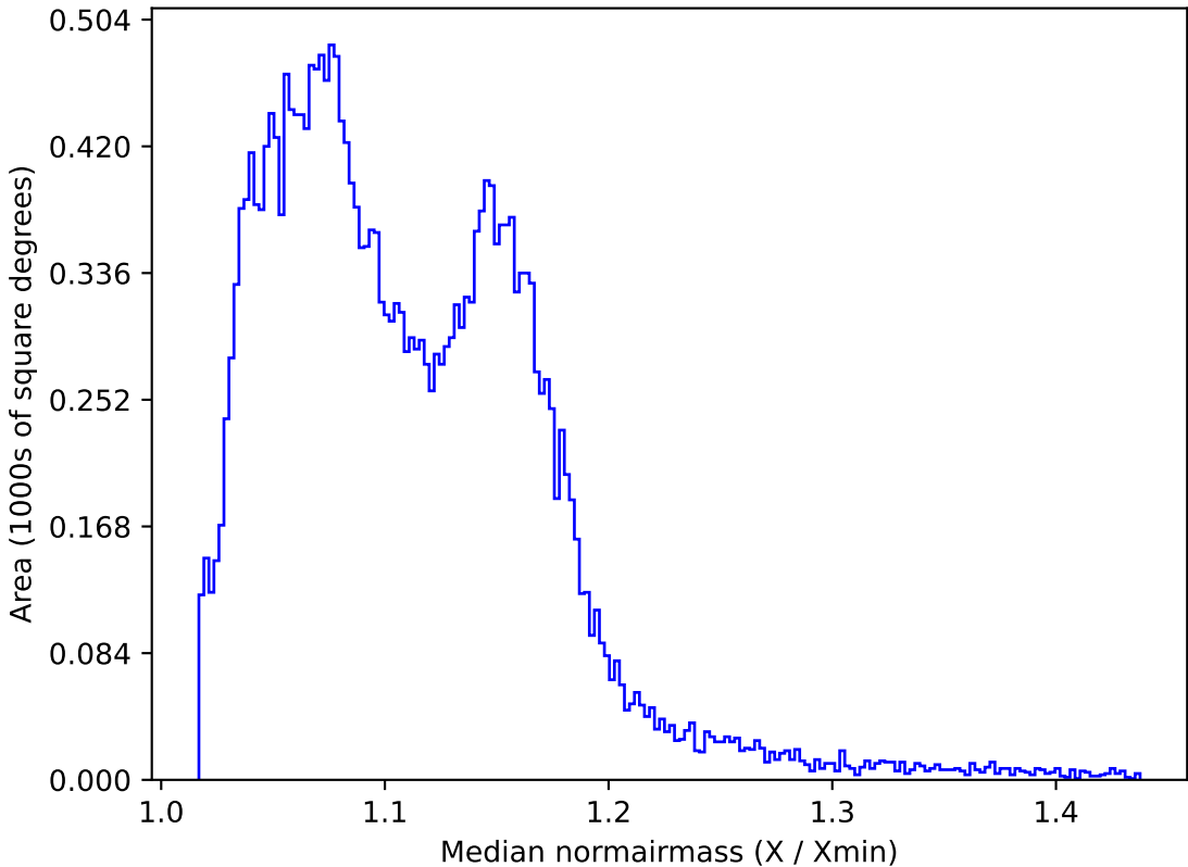
weather_cloudso35v3.4_10yrs All sky z band: Median normairmass
