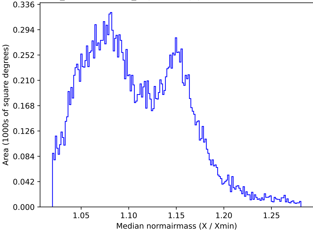
weather_cloudso35v3.4_10yrs All sky y band: Median normairmass
