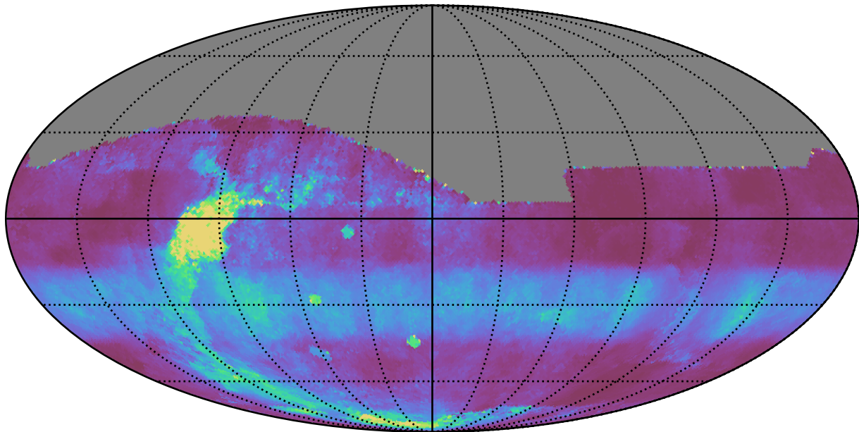
weather_cloudso35v3.4_10yrs All sky r band: Median normairmass
