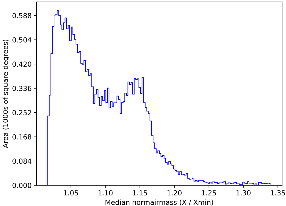
weather_cloudso35v3.4_10yrs All sky r band: Median normairmass
