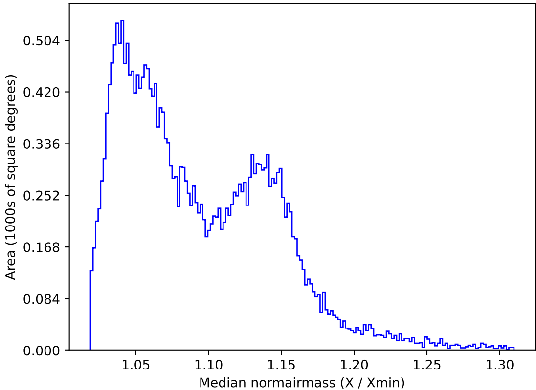
weather_cloudso35v3.4_10yrs All sky i band: Median normairmass
