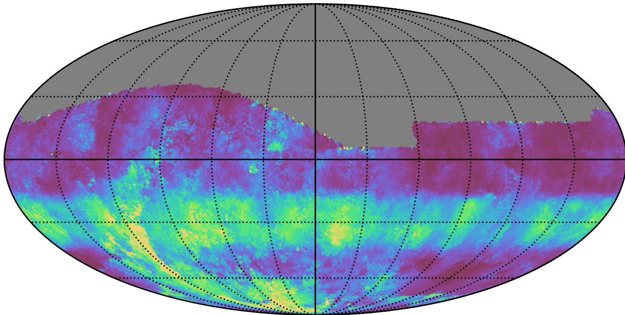
weather_cloudso35v3.4_10yrs All sky g band: Median normairmass
