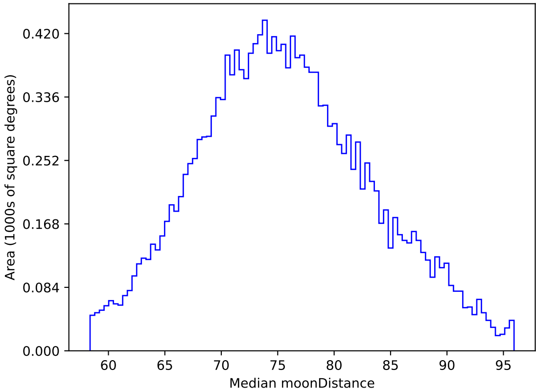
weather_cloudso35v3.4_10yrs WFD z band: Median moonDistance
