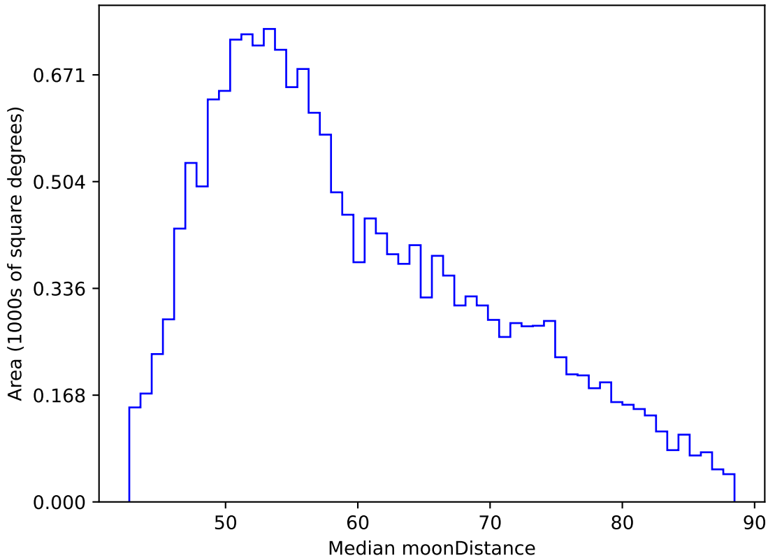
weather_cloudso35v3.4_10yrs WFD y band: Median moonDistance
