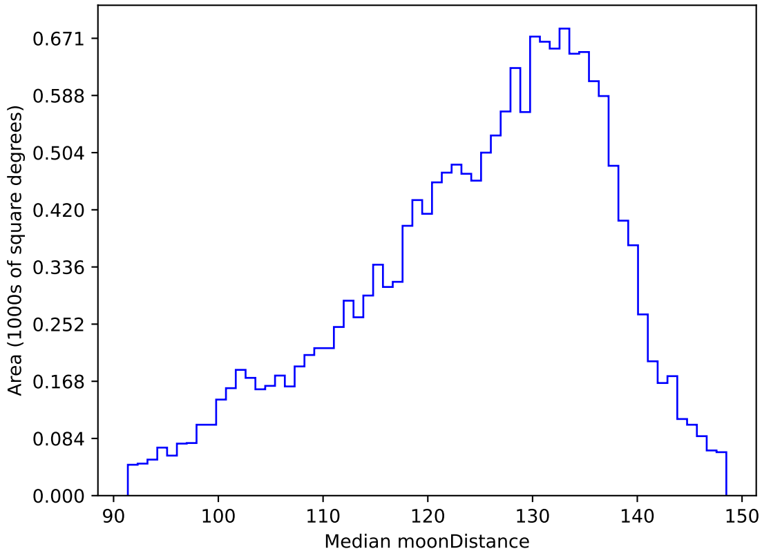
weather_cloudso35v3.4_10yrs WFD u band: Median moonDistance
