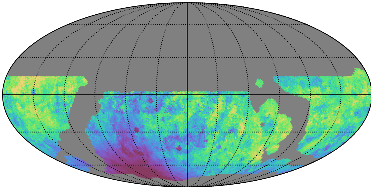
weather_cloudso35v3.4_10yrs WFD r band: Median moonDistance
