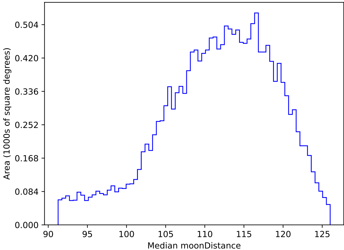
weather_cloudso35v3.4_10yrs WFD r band: Median moonDistance
