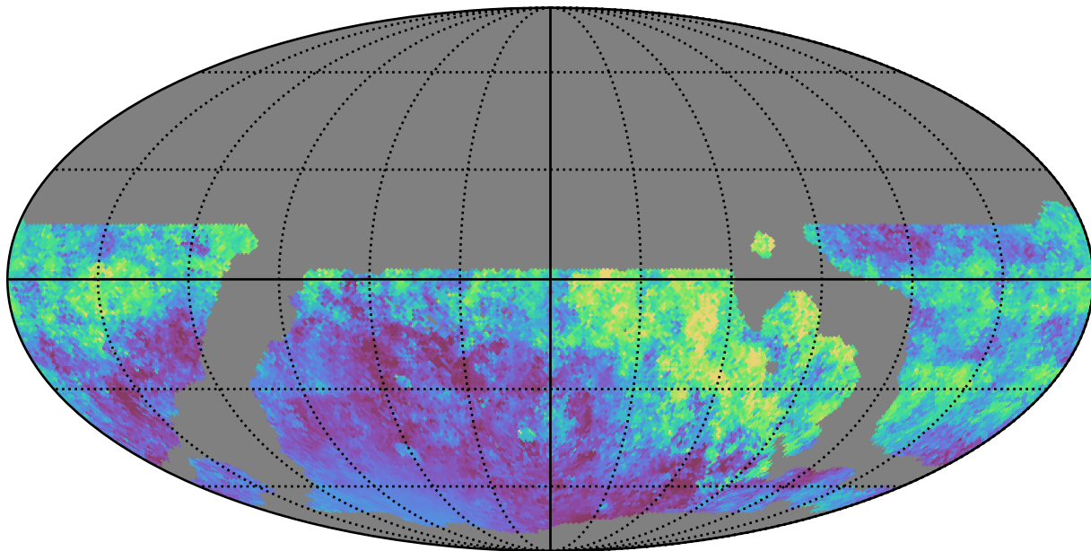
weather_cloudso35v3.4_10yrs WFD i band: Median moonDistance
