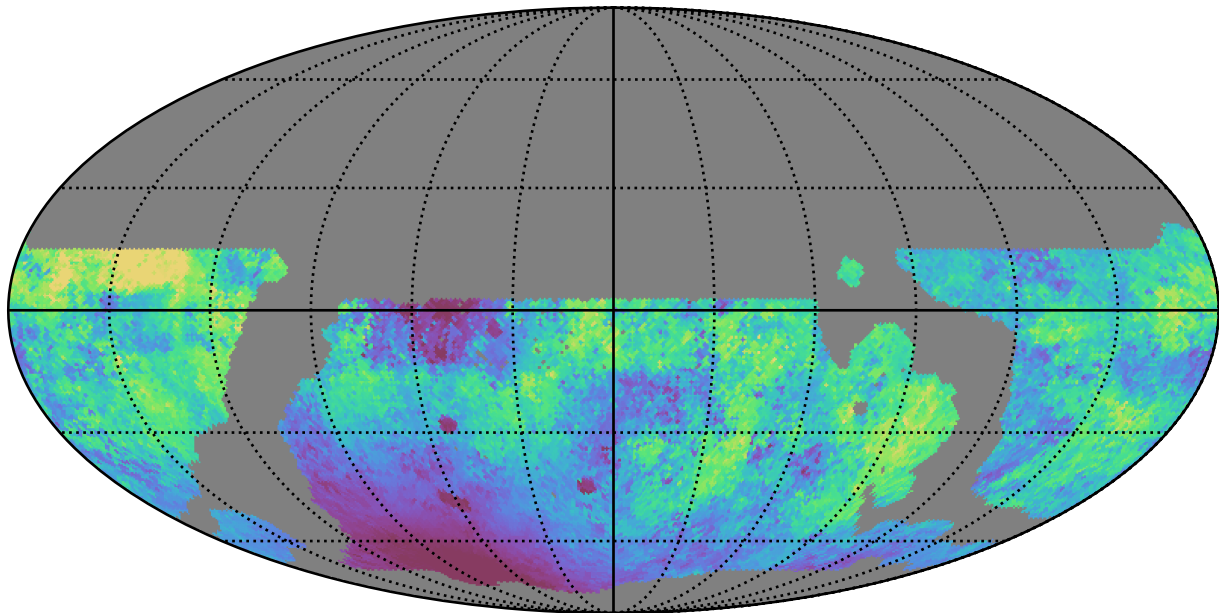
weather_cloudso35v3.4_10yrs WFD g band: Median moonDistance
