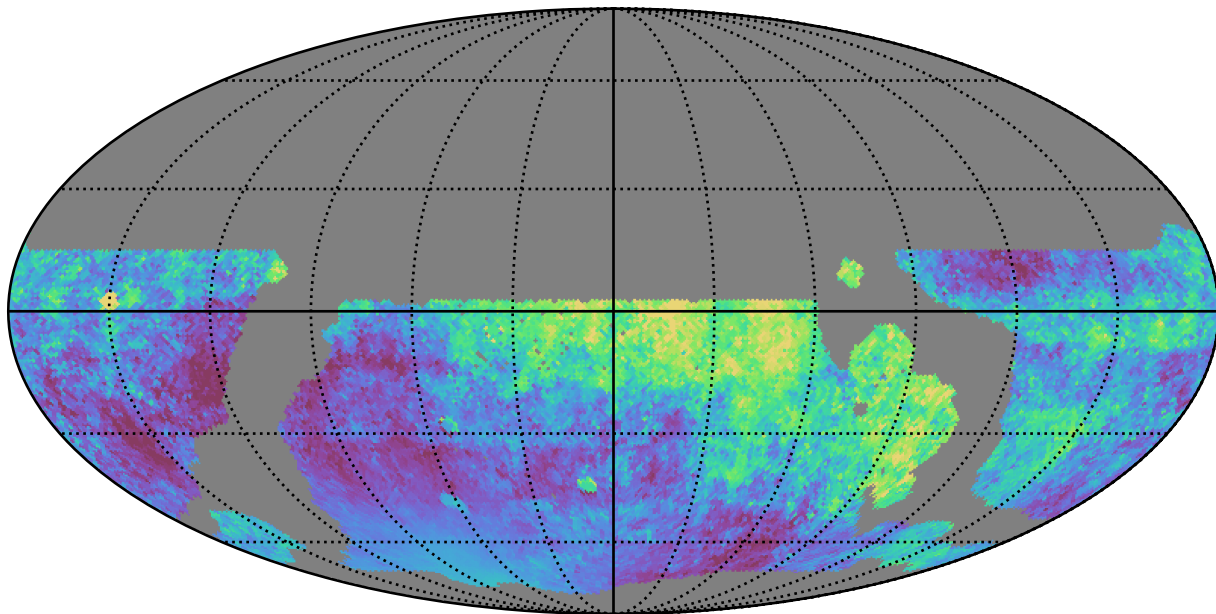
weather_cloudso35v3.4_10yrs WFD all bands: Median moonDistance
