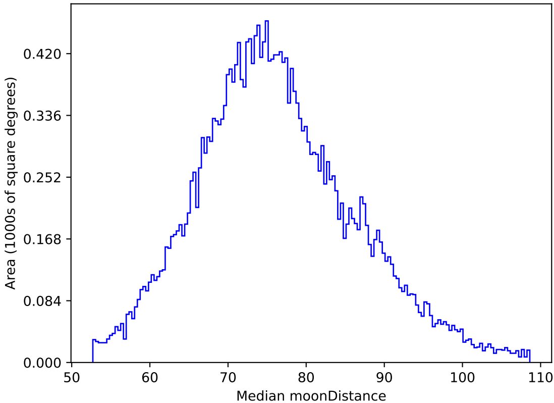
weather_cloudso35v3.4_10yrs All sky z band: Median moonDistance
