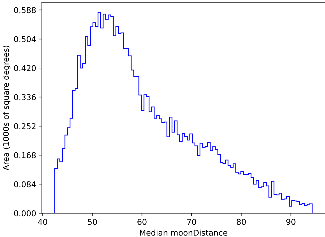
weather_cloudso35v3.4_10yrs All sky y band: Median moonDistance
