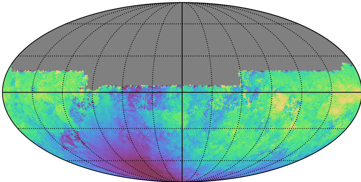
weather_cloudso35v3.4_10yrs All sky u band: Median moonDistance
