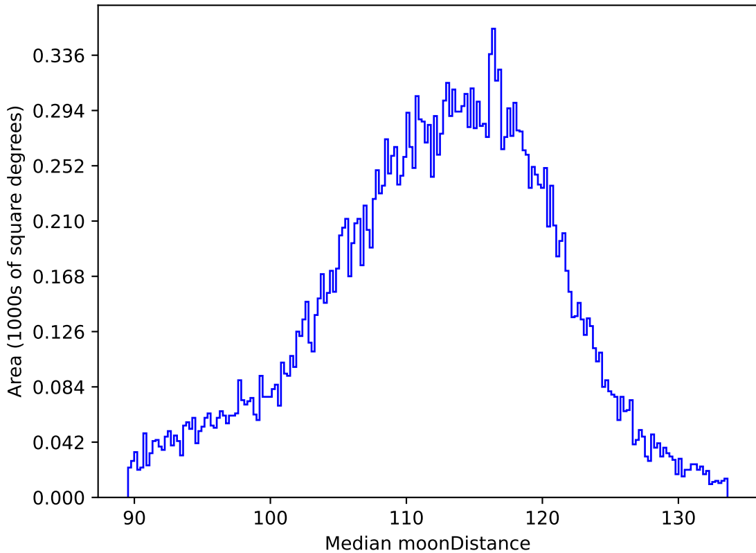
weather_cloudso35v3.4_10yrs All sky r band: Median moonDistance
