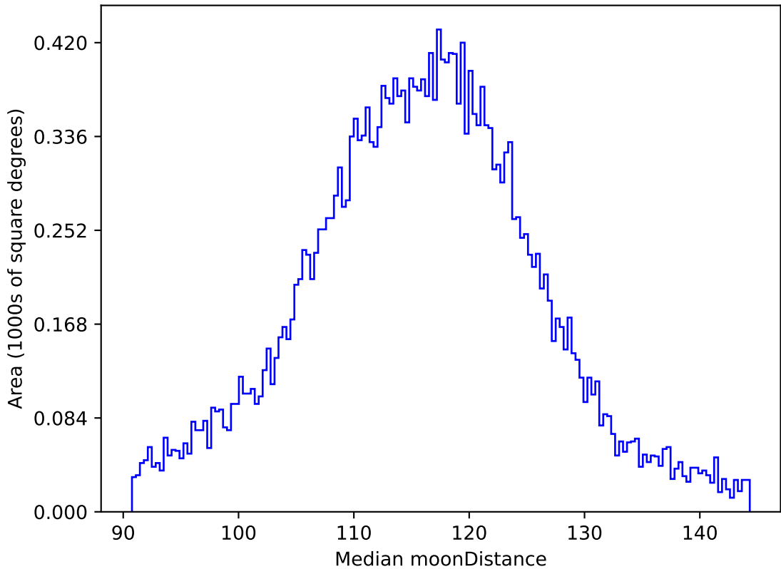
weather_cloudso35v3.4_10yrs All sky g band: Median moonDistance
