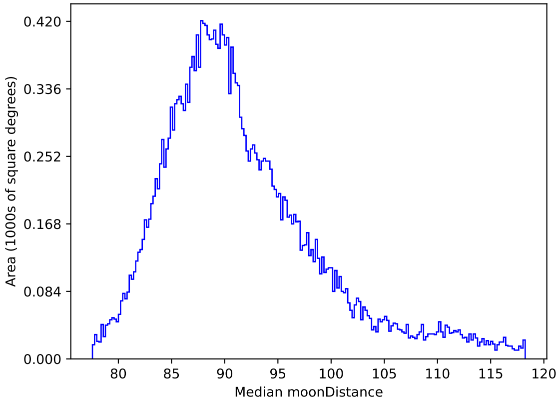
weather_cloudso35v3.4_10yrs All sky all bands: Median moonDistance
