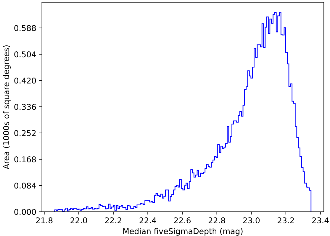
weather_cloudso35v3.4_10yrs Yr 1 z band: Median fiveSigmaDepth
