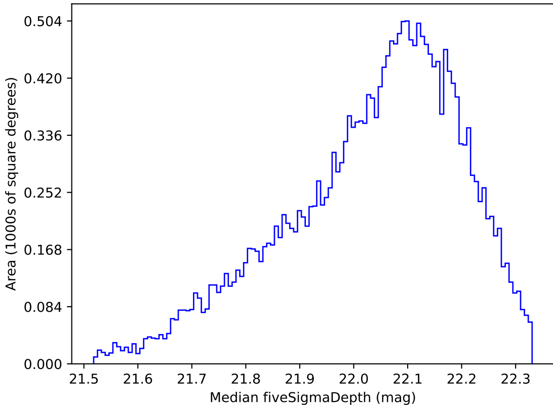
weather_cloudso35v3.4_10yrs Yr 1 y band: Median fiveSigmaDepth
