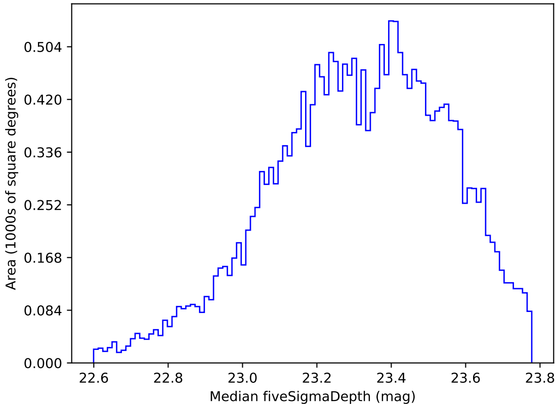
weather_cloudso35v3.4_10yrs Yr 1 u band: Median fiveSigmaDepth
