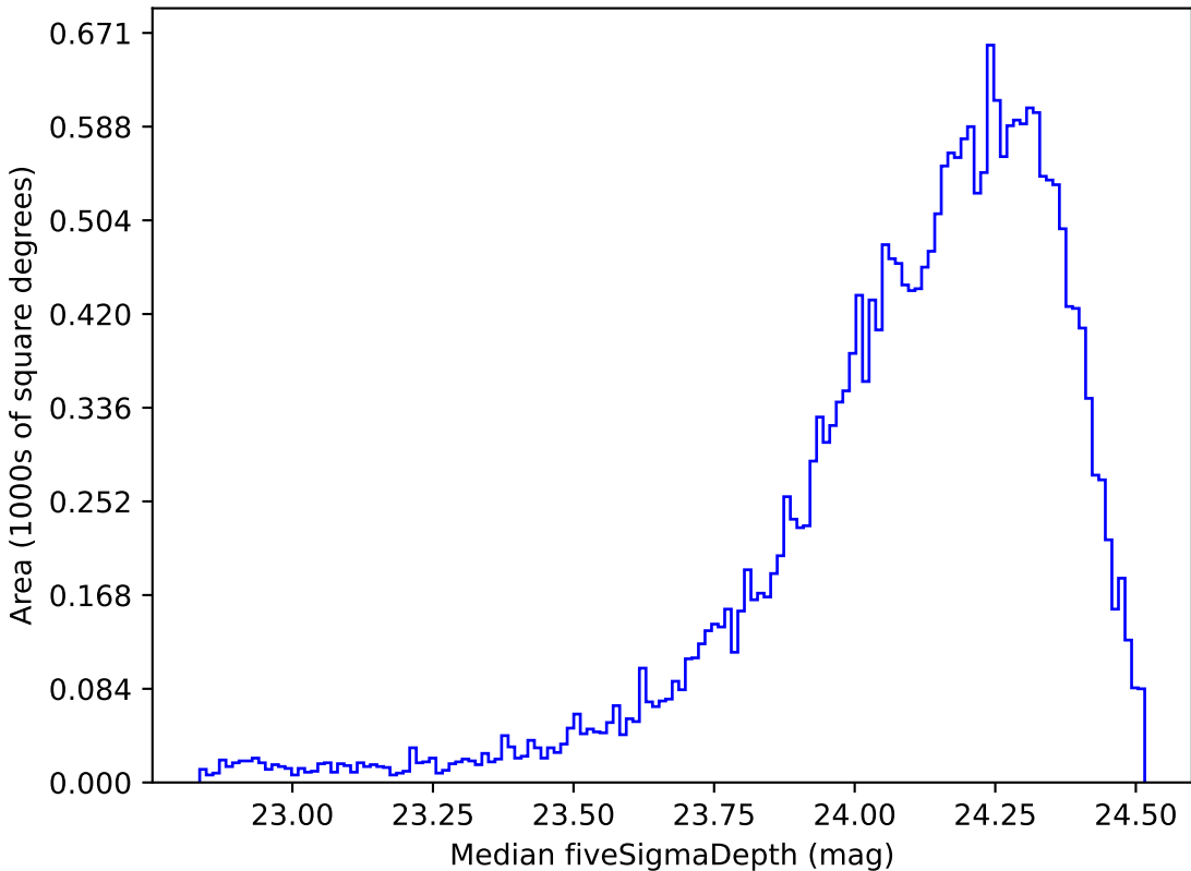
weather_cloudso35v3.4_10yrs Yr 1 r band: Median fiveSigmaDepth
