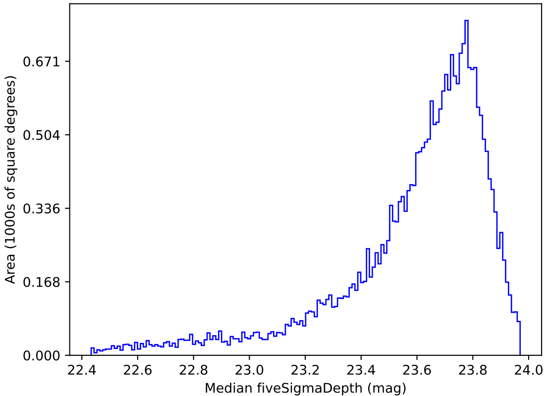
weather_cloudso35v3.4_10yrs Yr 1 i band: Median fiveSigmaDepth
