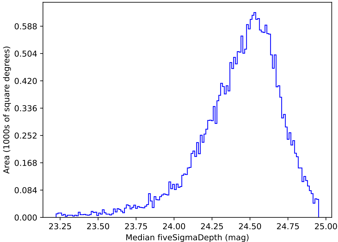
weather_cloudso35v3.4_10yrs Yr 1 g band: Median fiveSigmaDepth
