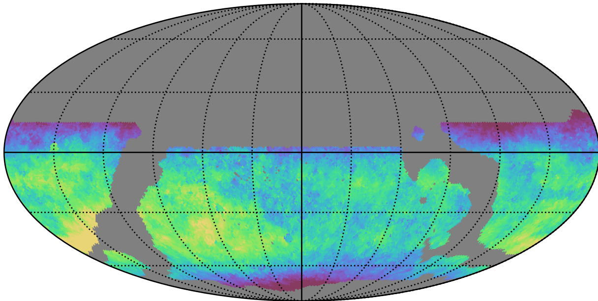
weather_cloudso35v3.4_10yrs WFD z band: Median fiveSigmaDepth
