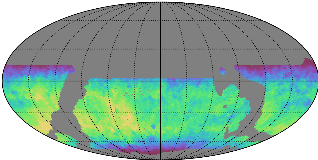
weather_cloudso35v3.4_10yrs WFD y band: Median fiveSigmaDepth
