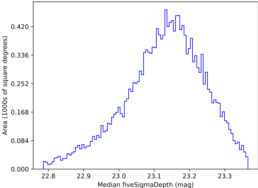
weather_cloudso35v3.4_10yrs WFD u band: Median fiveSigmaDepth
