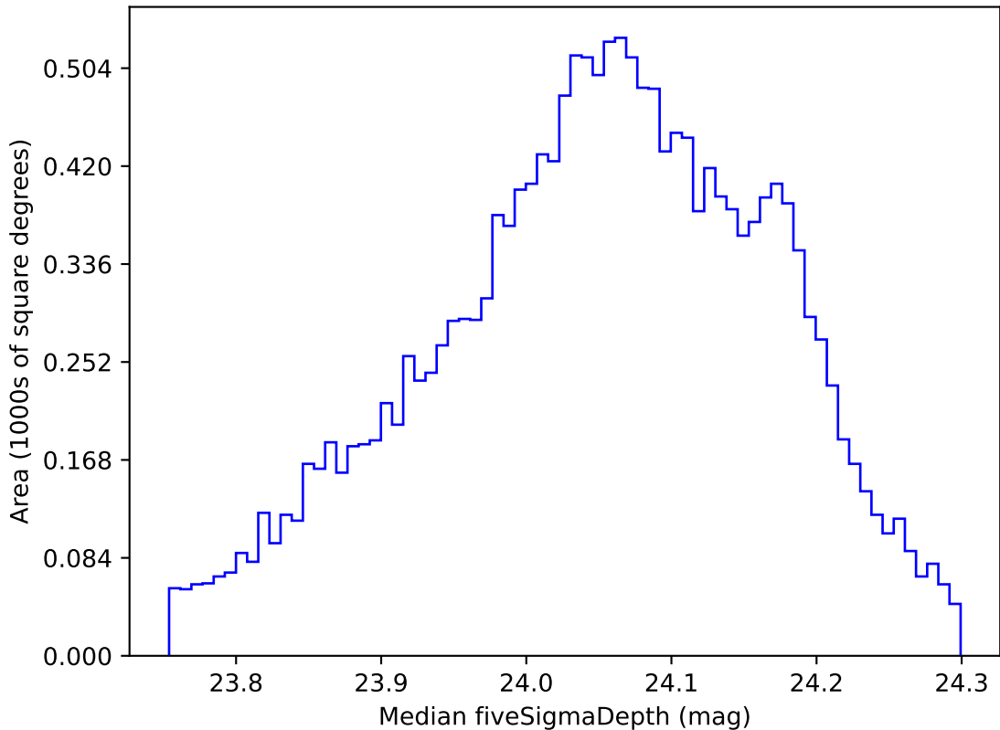
weather_cloudso35v3.4_10yrs WFD r band: Median fiveSigmaDepth
