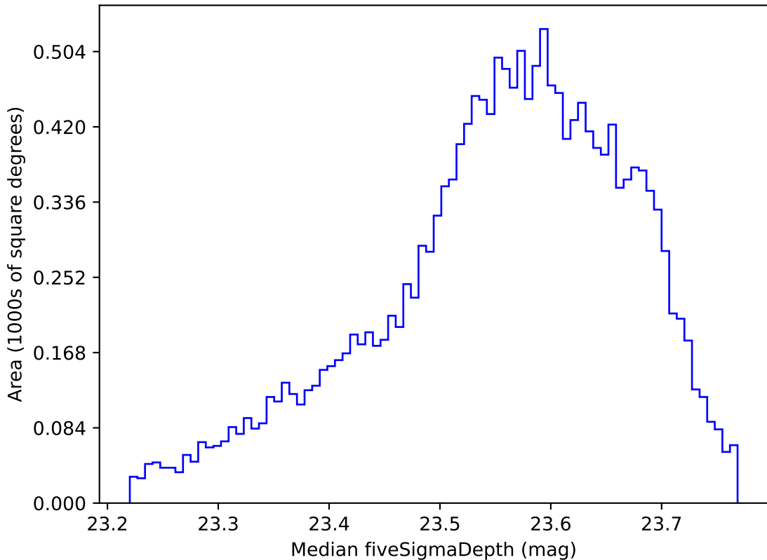
weather_cloudso35v3.4_10yrs WFD i band: Median fiveSigmaDepth
