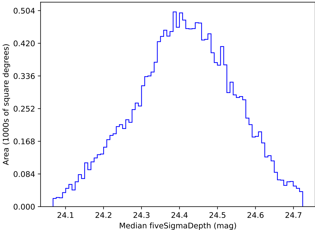
weather_cloudso35v3.4_10yrs WFD g band: Median fiveSigmaDepth
