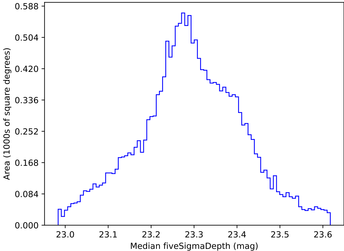
weather_cloudso35v3.4_10yrs WFD all bands: Median fiveSigmaDepth
