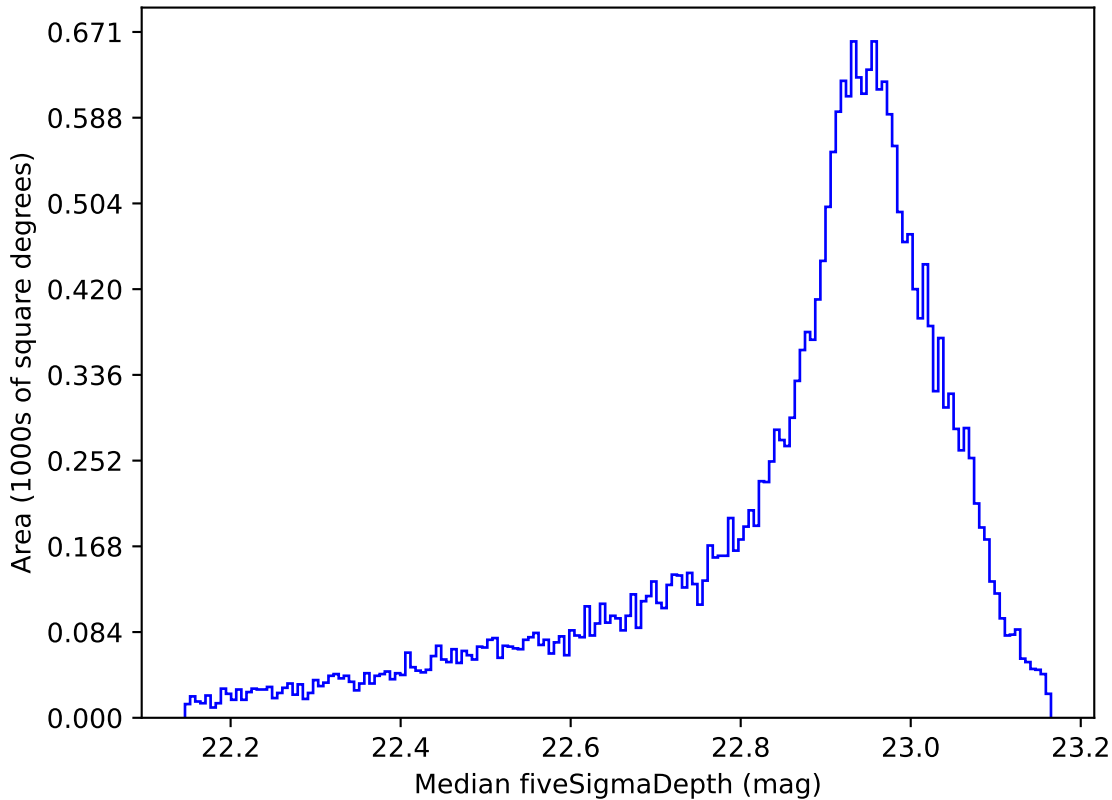
weather_cloudso35v3.4_10yrs All sky z band: Median fiveSigmaDepth
