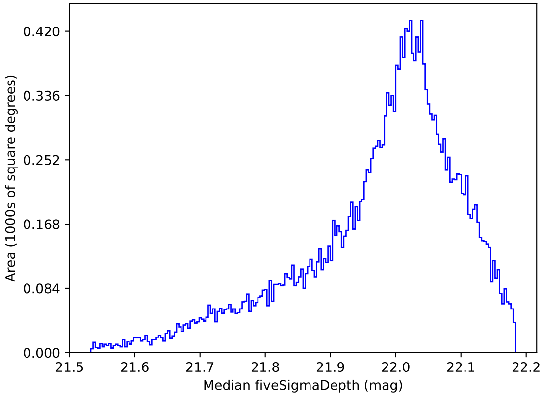
weather_cloudso35v3.4_10yrs All sky y band: Median fiveSigmaDepth
