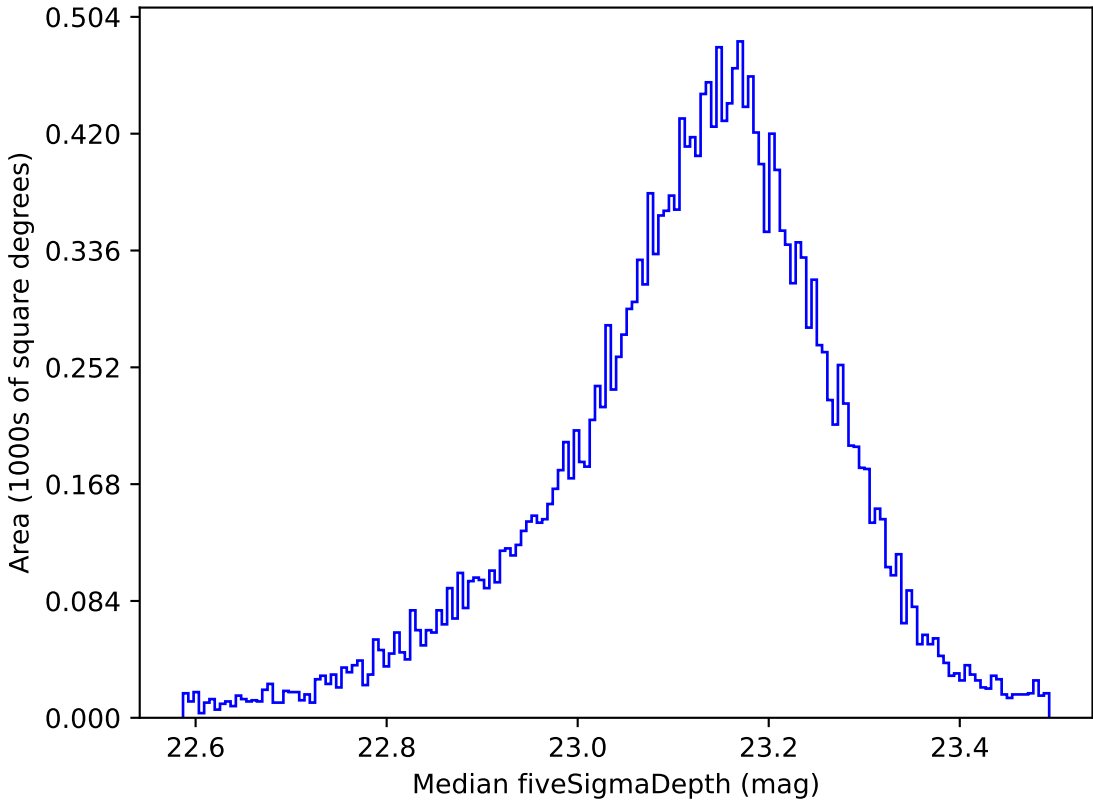
weather_cloudso35v3.4_10yrs All sky u band: Median fiveSigmaDepth
