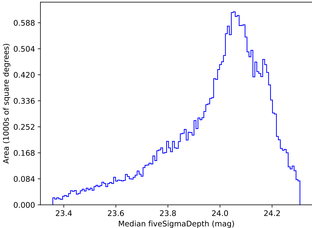
weather_cloudso35v3.4_10yrs All sky r band: Median fiveSigmaDepth
