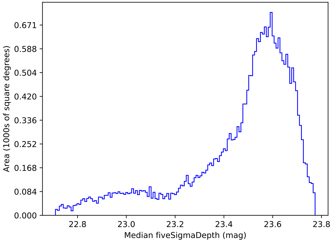
weather_cloudso35v3.4_10yrs All sky i band: Median fiveSigmaDepth
