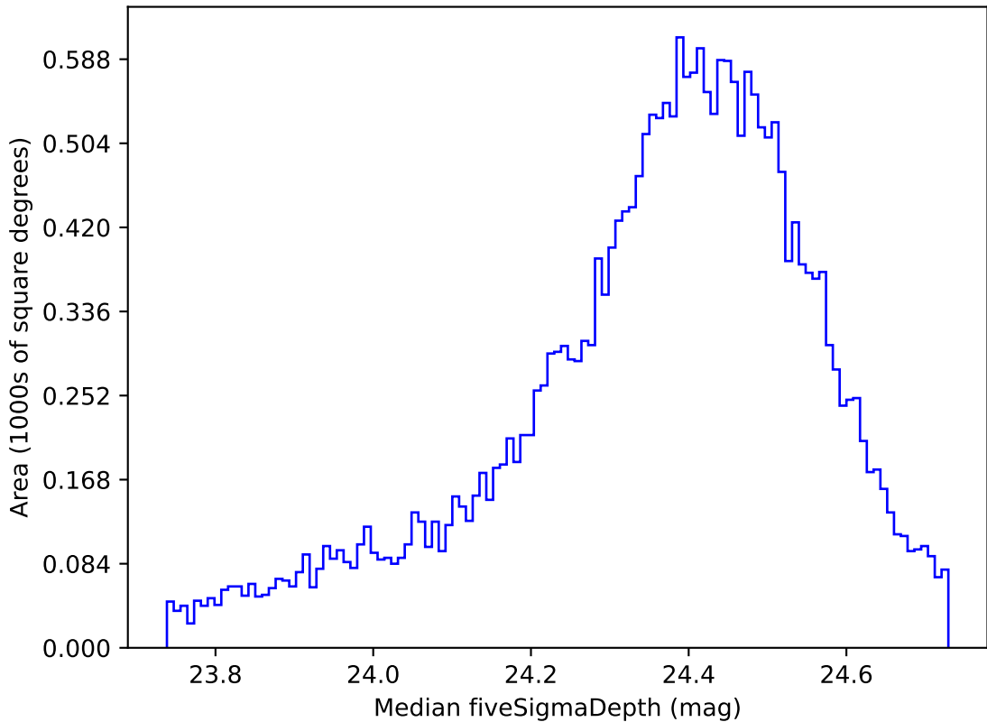
weather_cloudso35v3.4_10yrs All sky g band: Median fiveSigmaDepth
