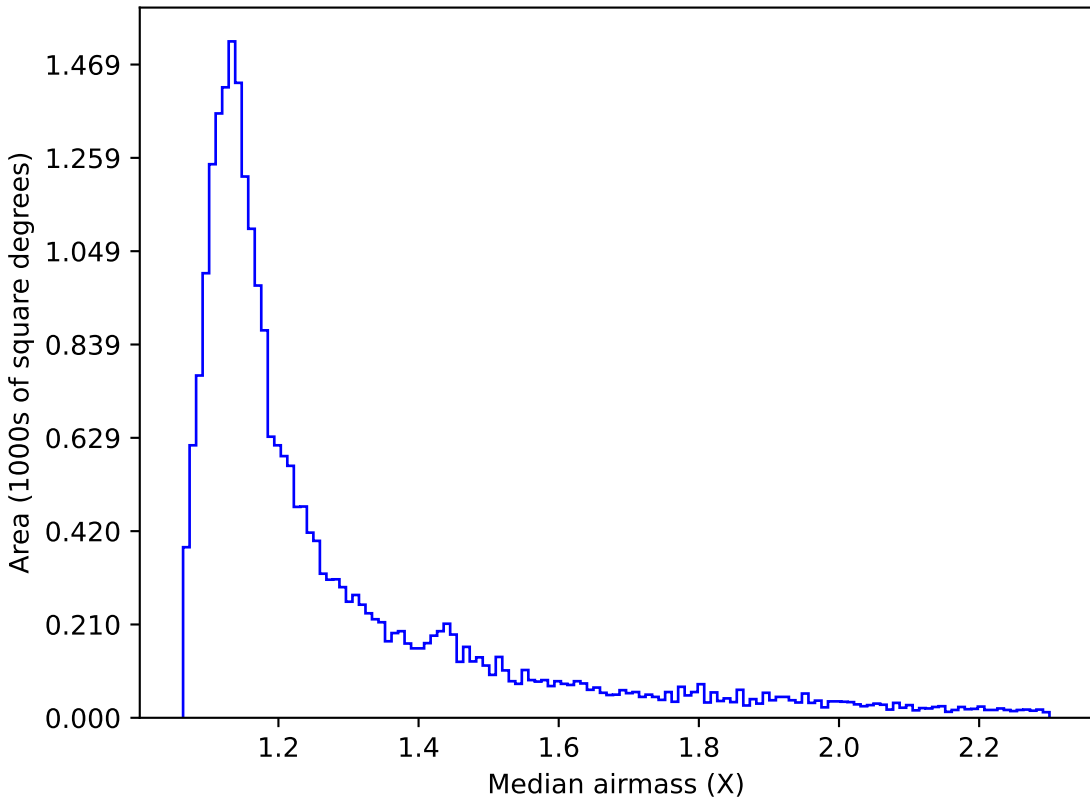
weather_cloudso35v3.4_10yrs Yr 1 z band: Median airmass
