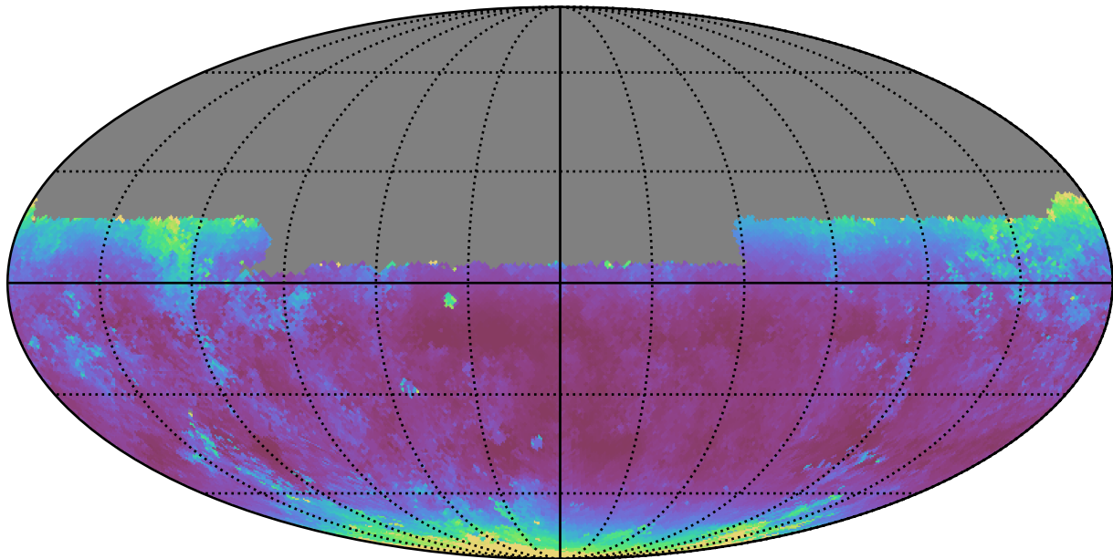
weather_cloudso35v3.4_10yrs Yr 1 y band: Median airmass
