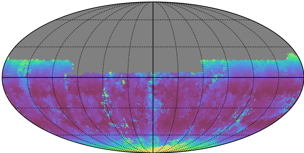
weather_cloudso35v3.4_10yrs Yr 1 u band: Median airmass
