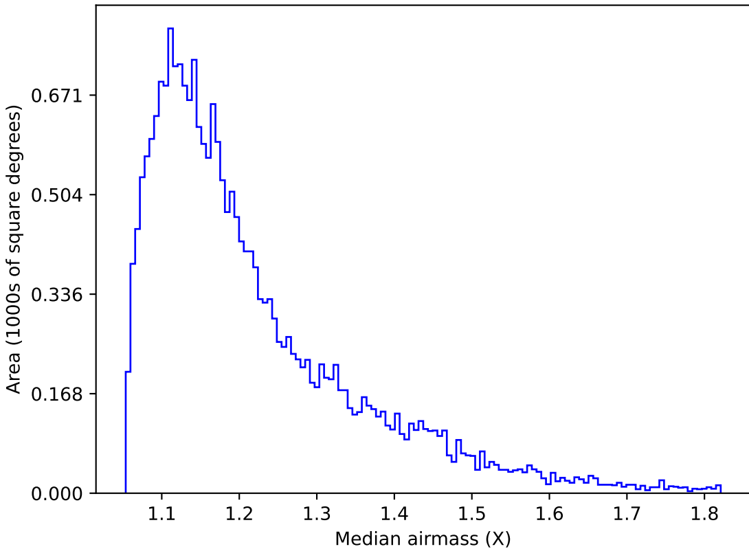
weather_cloudso35v3.4_10yrs Yr 1 u band: Median airmass
